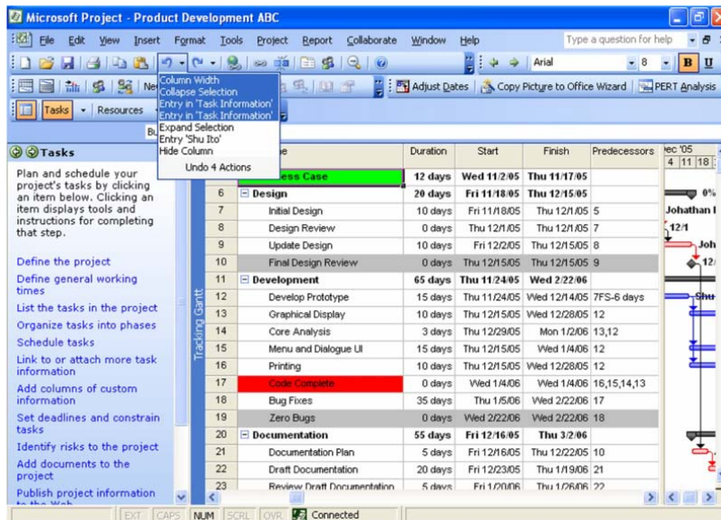
Figure 3: Expanded Multi-Level Undo menu
